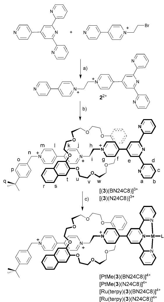
Scheme 2. a) MeCN, reflux, 7 days; anion exchange with NaOTf. b) tert -Butylbenzylbromide (2 equiv), crown ether (6 equiv), MeCN, RT, 7 days; anion exchange with NaOTf. c) For Pt complexes: [\text{PtClMe}(\text{Me}_2\text{S})_2] and AgOTf (1 equiv of each), MeOH, 50 °C, 24 h; for Ru complexes: [\text{RuCl}_3(\text{terpy})] , reflux in EtOH/H 2 O, 12 h; labels refer to NMR spectral assignments. All anions are OTf − .
